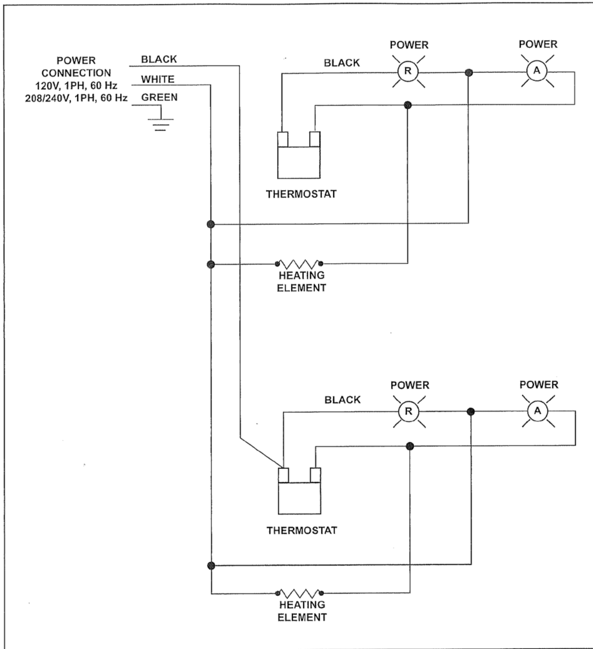
VBP77I Wiring Diagram
