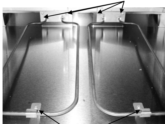
ELEMENT CLIP SCREWS
