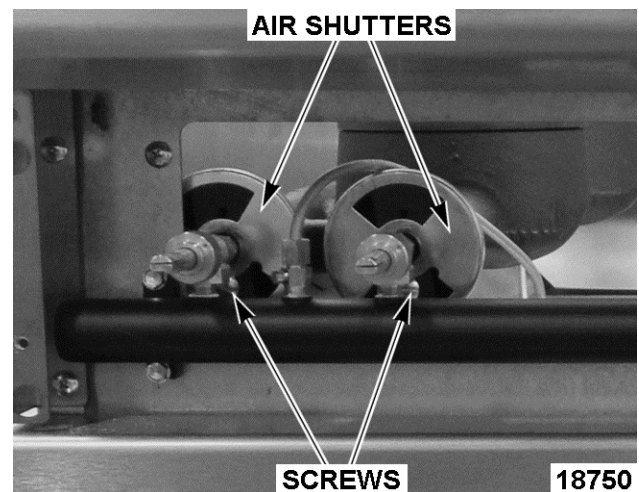
Top Burner Air Shutters
