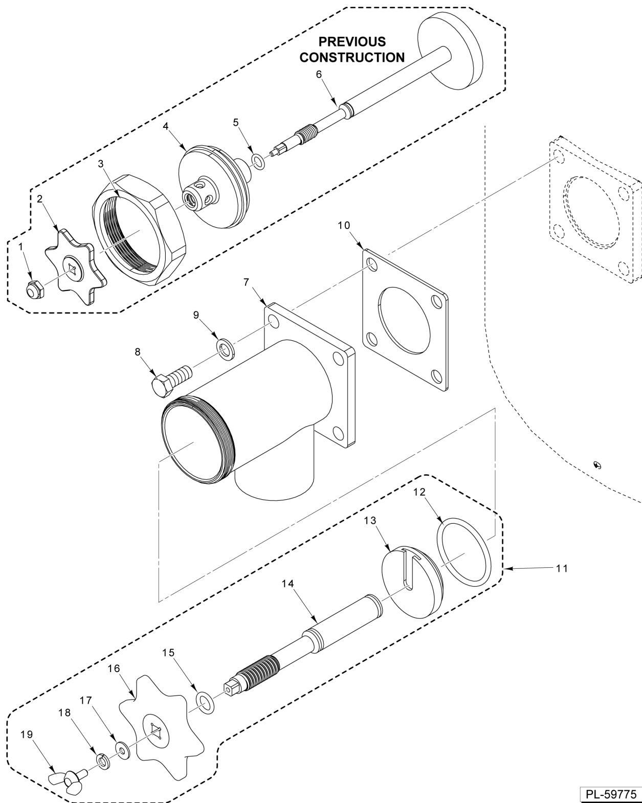
DRAW-OFF VALVE ASSEMBLY (3 INCH)
