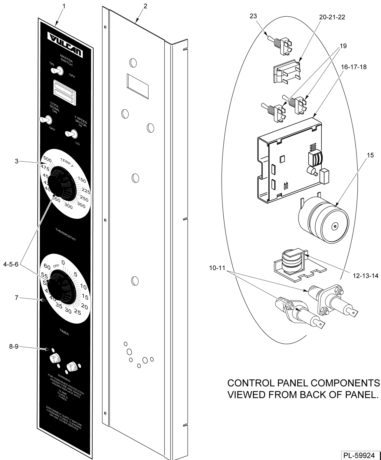
CONTROL PANEL (ECO2D) (PREVIOUS CONSTRUCTION) (PRIOR TO FEBRUARY 2003)
