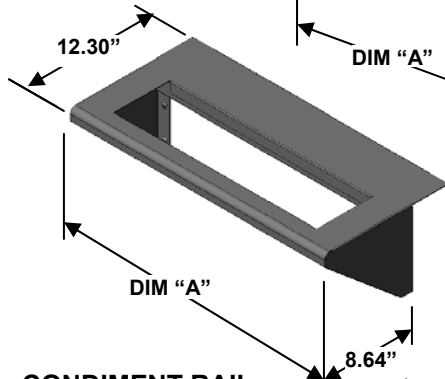
CONDIMENT RAIL
