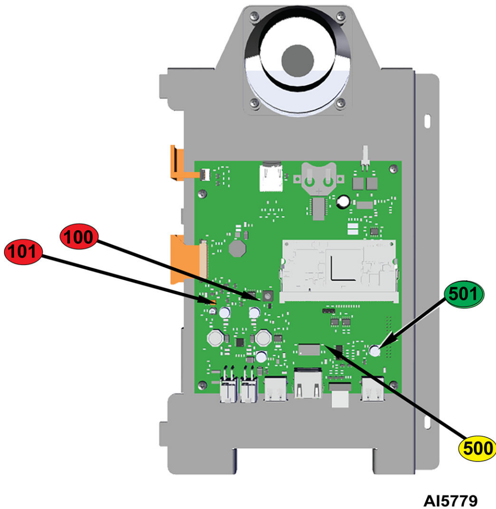
Fig. 174 INTERFACE BOARD
