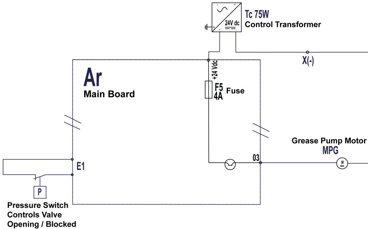
CHEF Combi Grease Collection Diagram DERIVED FROM Option Collection graisse_Grease collection option Rev A
