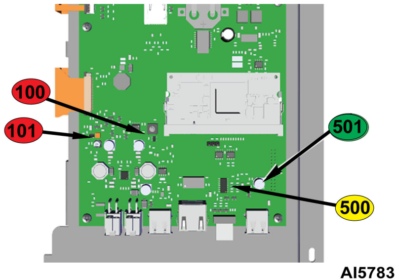
Fig. 176 INTERFACE BOARD
