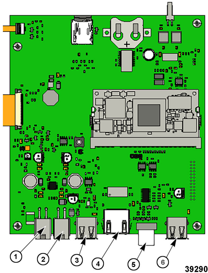
Fig. 183 INTERFACE BOARD
