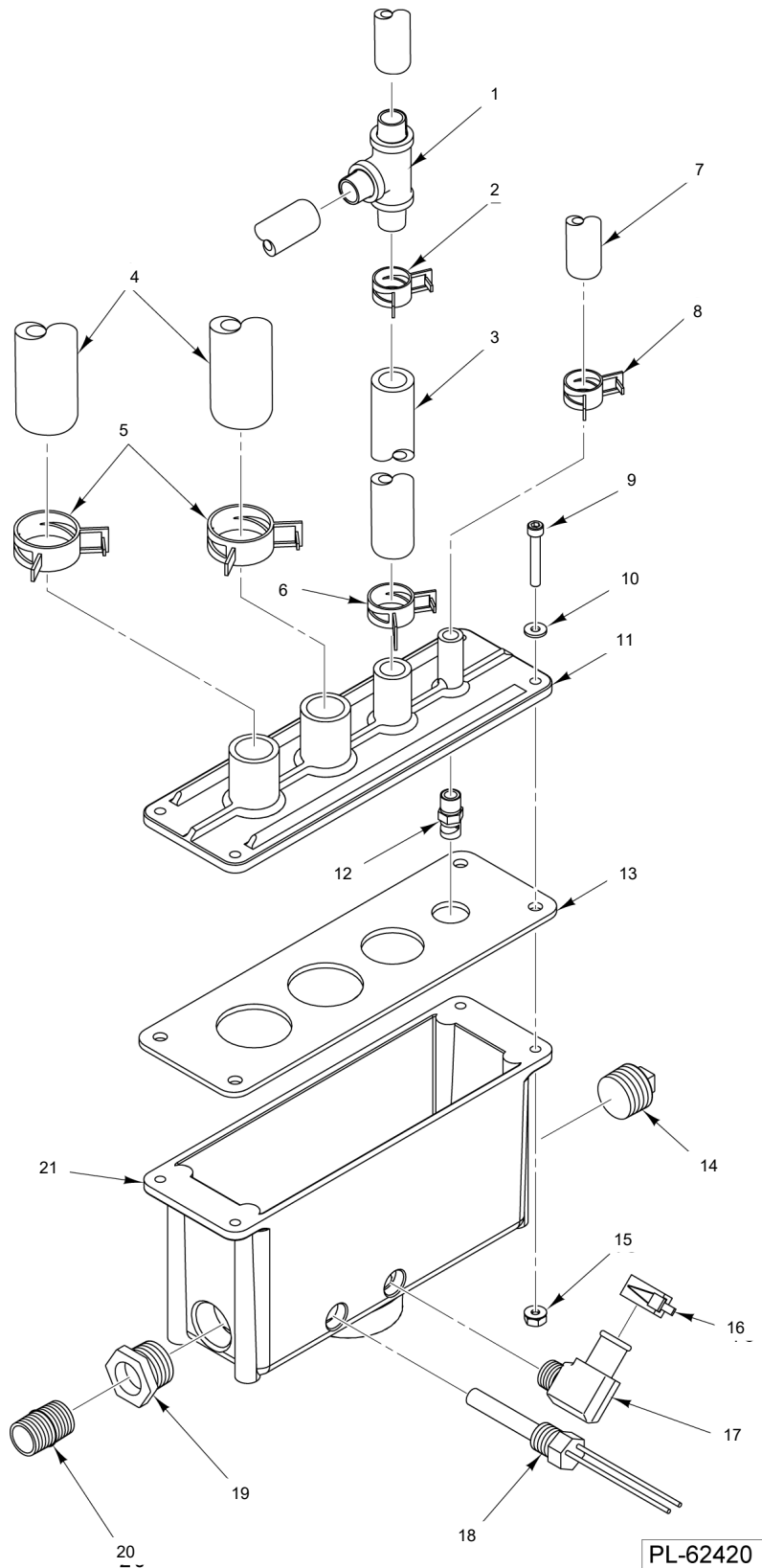
DRAIN ASSEMBLY
