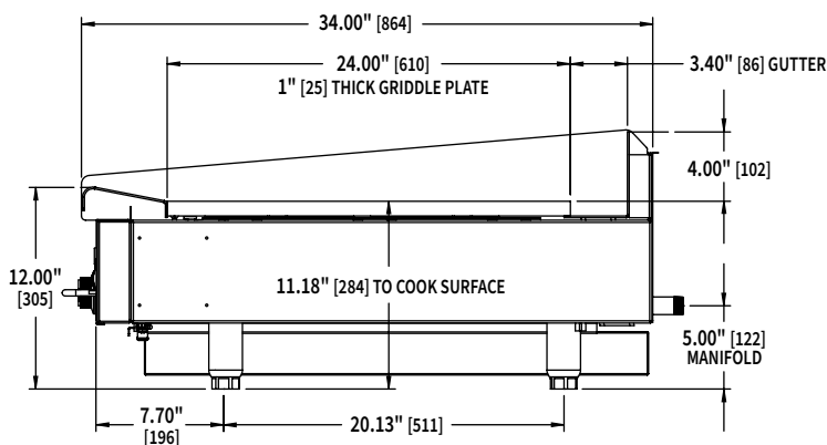
Rear Grease Trough - Side View
