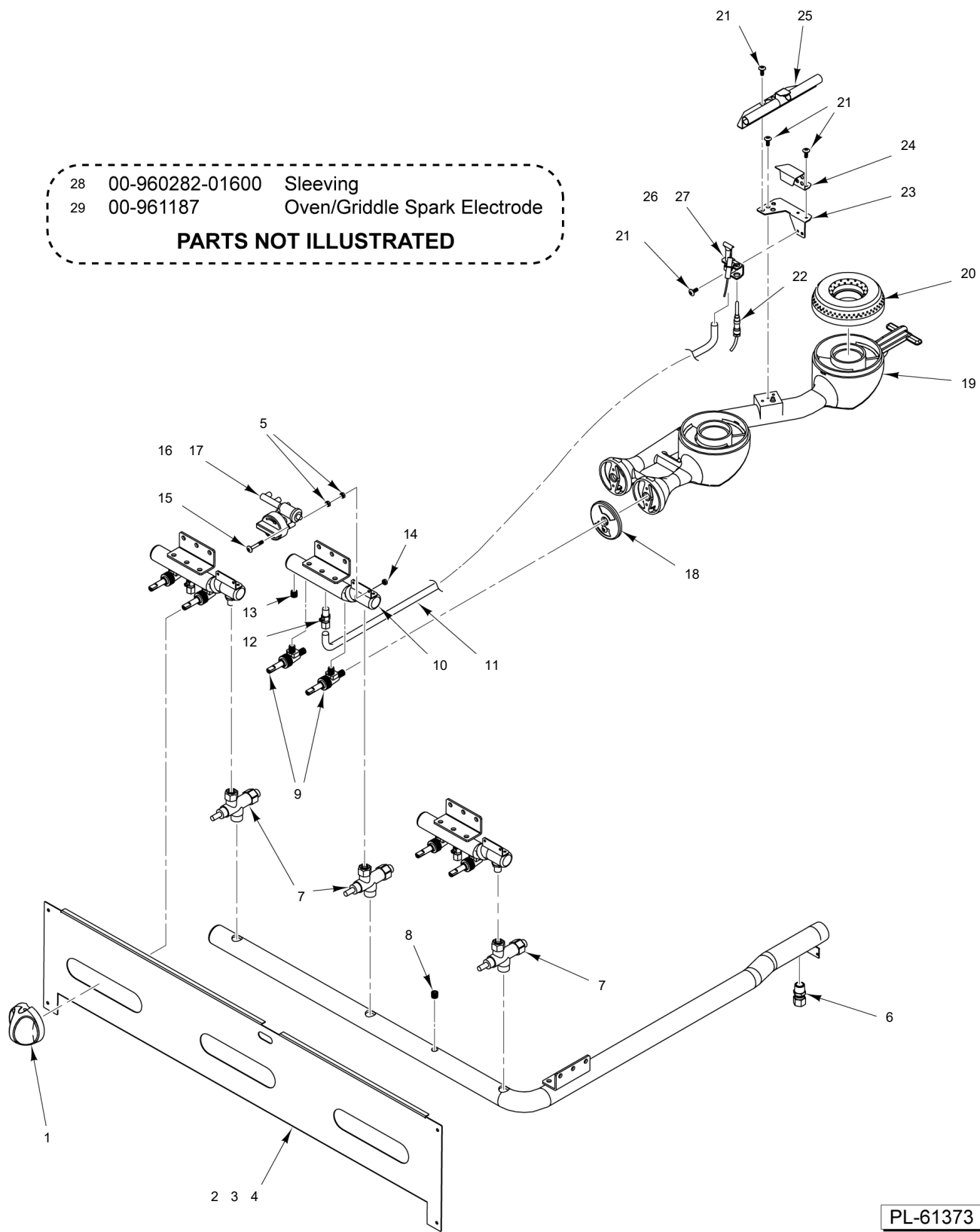
TOP BURNER & MANIFOLD (FLAME SAFETY OPTION)
