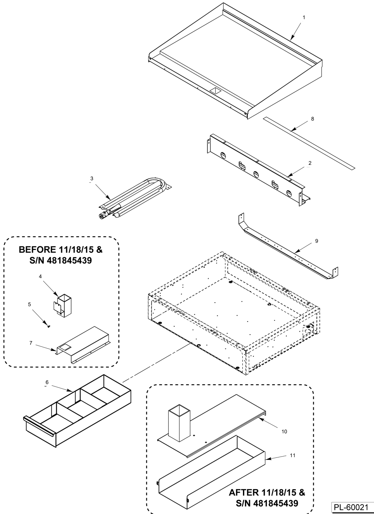
GRIDDLE TOP MODULE (36 INCH) (BEFORE S/N 481938362)
