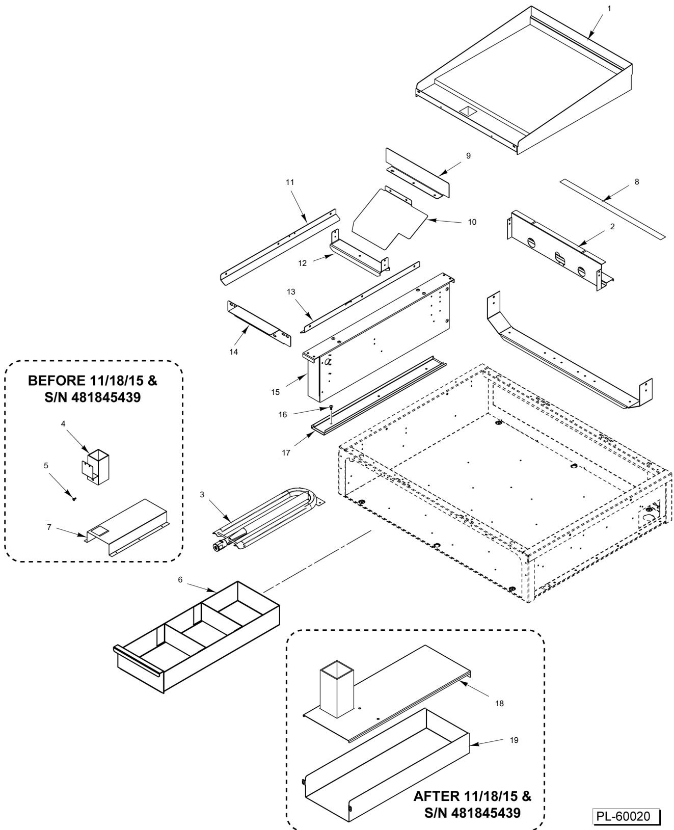
GRIDDLE TOP MODULE (24 INCH) (BEFORE S/N 481938362)
