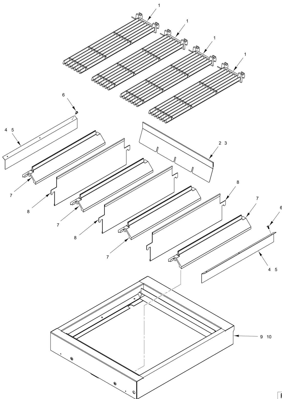
CHARBROILER GRILL
