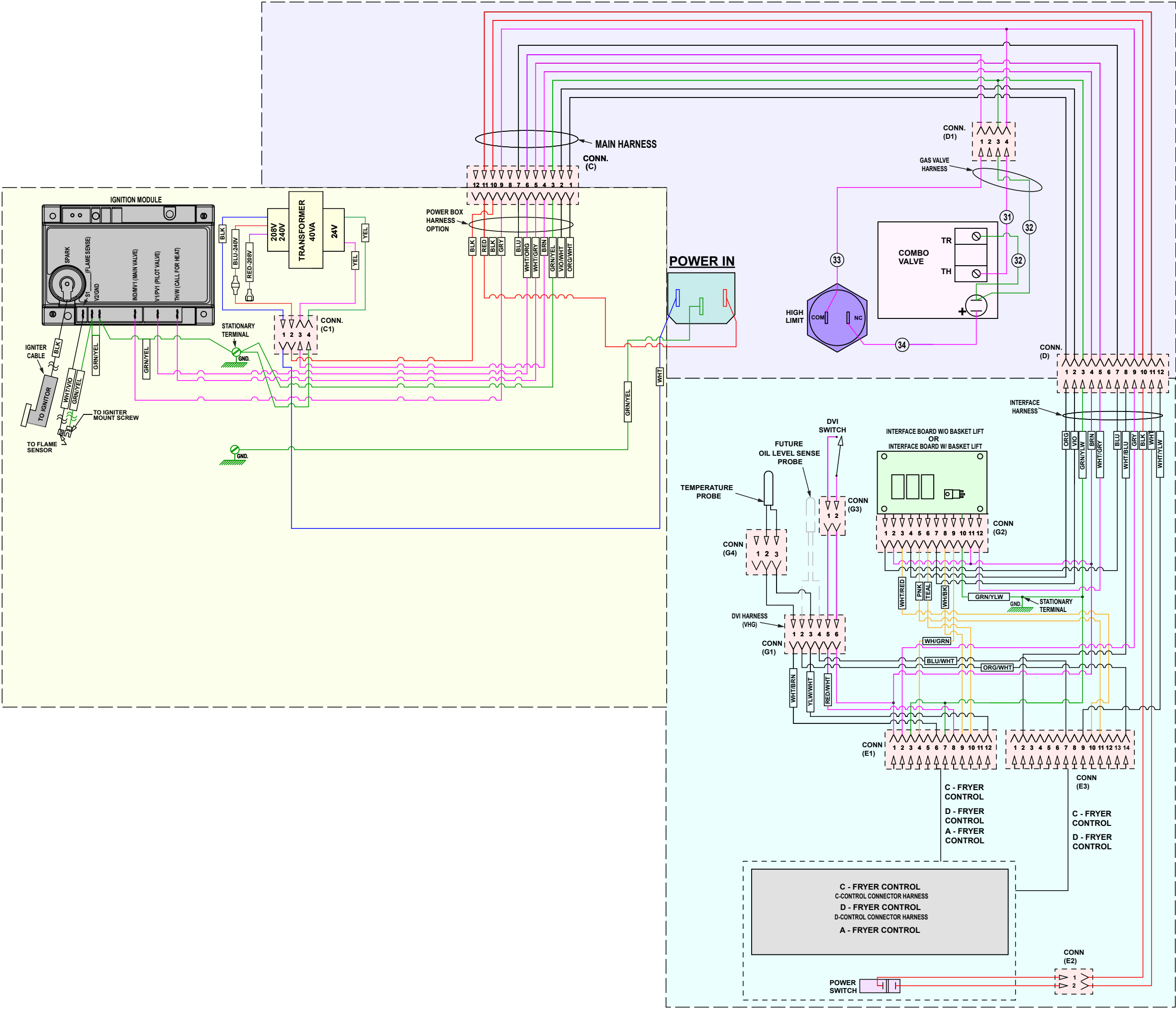
WIRING DIAGRAM, VH G FRYER OPTION HARNESS, 240VAC, 1PH VH G A MODEL VH G D MODEL VH G C MODEL 976718-1 REV. G
