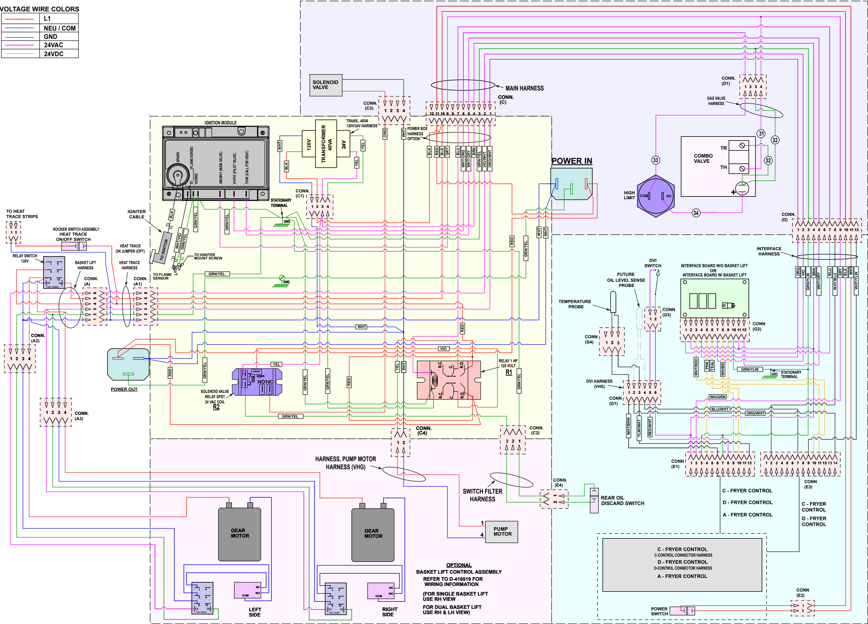
WIRING DIAGRAM, VHG FRYER OPTION HARNESS, 120VAC, 1PH
