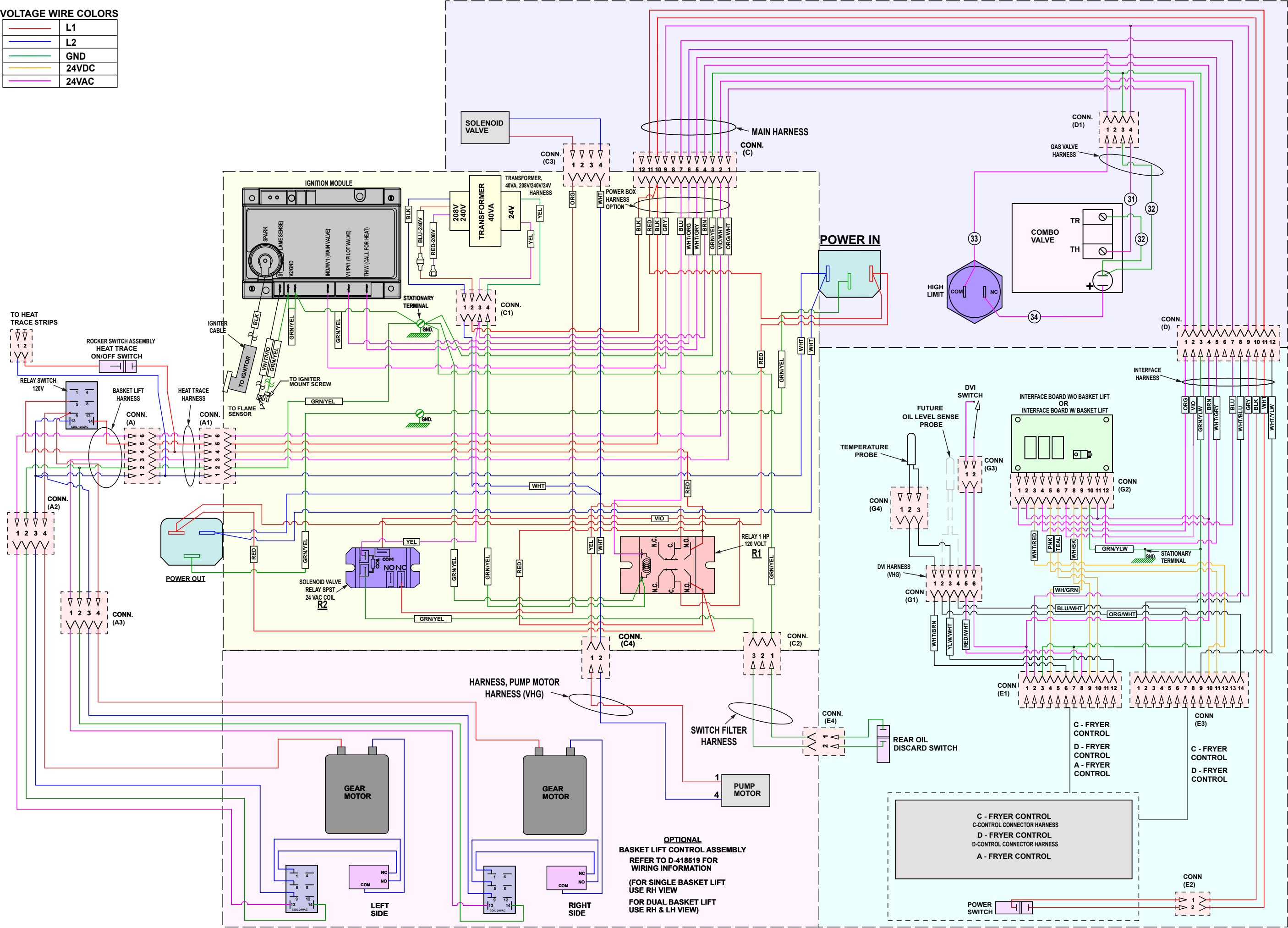
WIRING DIAGRAM, VHG FRYER OPTION HARNESS, 240VAC, 1PH VHG A MODEL VHG D MODEL VHG C MODEL 976718-1 REV. G
