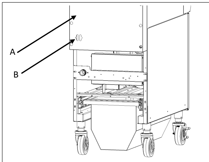
A Rear Of Fryer B Strain Relief Chan Connection (Chain supplied by others)
