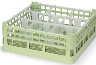
52763 9-COMPARTMENT 5 5 / 8 " (14.9 cm) sq. compartment 8 1 / 16 " (21.1 cm) diagonal
