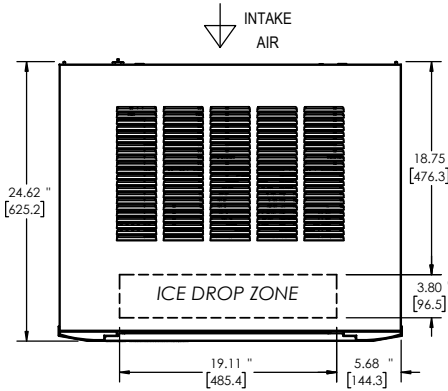
PLAN / TOP VIEW
