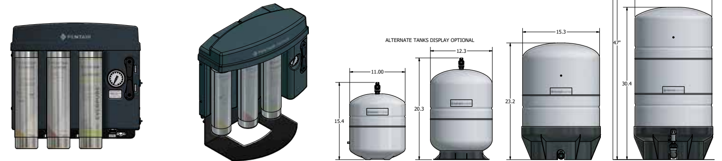
Wall-mounted EZ-RO processor EZ-RO on (optional) floor stand Hydro-pneumatic tank sizes, depending on model purchased: 2 gal, 5 gal, 10 gal, 16 gal
