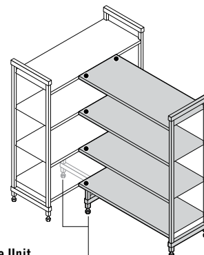
Starter + Add-On Unit With Shared Post
