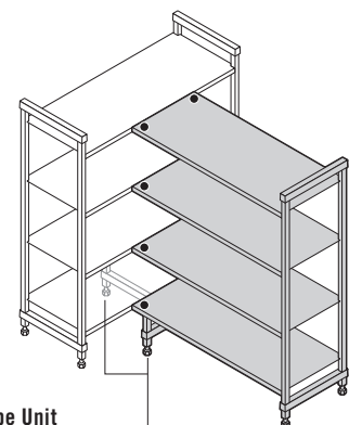
T-Shape Unit Starter unit + Add-on unit using 1 set of corner connectors per shelf and 2 dunnage stands.
