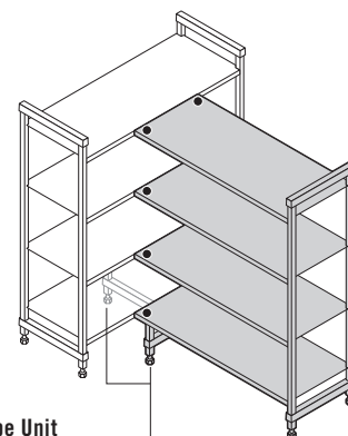
T-Shape Unit Starter unit + Add-on unit using 1 set of corner connectors per shelf and 2 dunnage stands.
