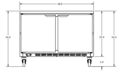
00C31-054A KIT - CASTER 36" WORK TOP HEIGHT, SPE/WT 401-249A/401-250A 00A31-030D-03 LEVELER
