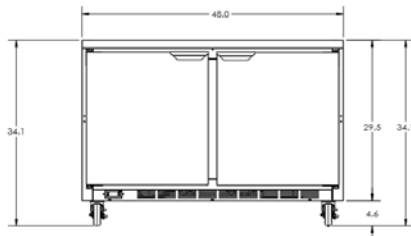
00A31-059A KIT - CASTER, SPE/WT 34-1/8" WORKTOP HEIGHT 411-006A / 411-007A
