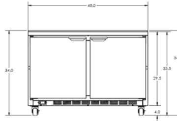
00A31-052A KIT - CASTER SPE, 34" CUTTING BRD HEIGHT 3" CASTERS / 500# 401-695A / 401-696A 00C31-032D-03 LEVELER
