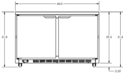
00C31-049A 2-3/4" CASTERS - "LOW PROFILE" 401-926D-01 / 401-926D-02
