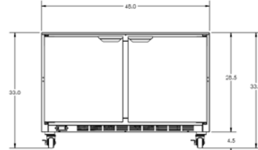
00A31-051A KIT - CASTER 3" WHEEL 3.75" HEIGHT 500 LB 401-633A / 401-634A 00A31-031D-03 LEVELER
