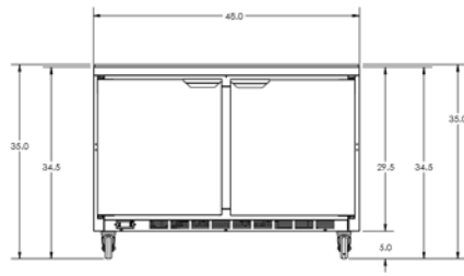
00A31-061A CASTER KIT-SPE/WT CUTTING BOARD HGT 35" 411-927D-01 / 401-927D-02 00A31-045D-03 LEVELER
