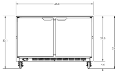
00A31-059A KIT - CASTER, SPE/WT 34-1/8" WORKTOP HEIGHT (UC-33-1/8") 411-006A / 411-007A
