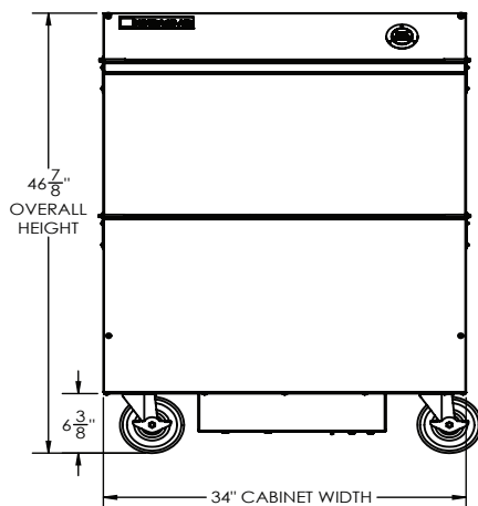
ELEVATION VIEW
