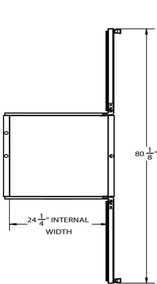
PLAN VIEW
