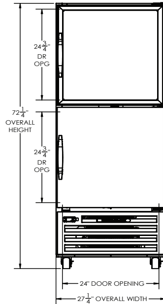
ELEVATION VIEW
