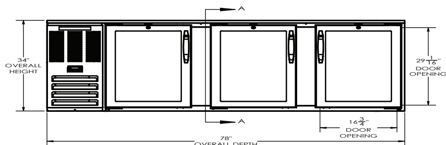
ELEVATION VIEW
