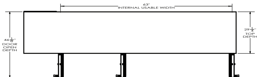
ELEVATION VIEW
