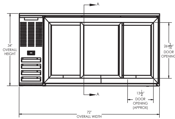
ELEVATION VIEW
