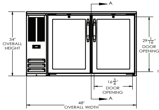
ELEVATION VIEW
