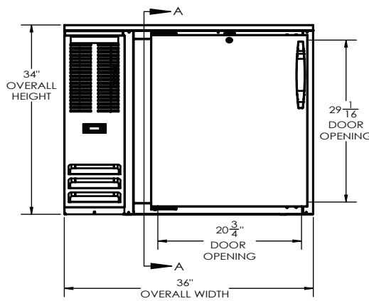
ELEVATION VIEW
