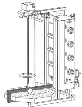
VB-5 WITH STABILIZING SUPPORT BAR FOR ADD WEIGHT
