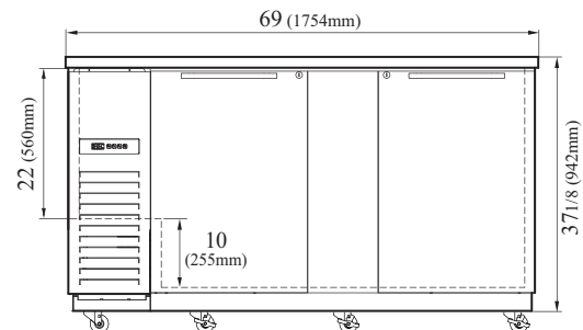
TBB-3SBD-N6 FRONT VIEW
