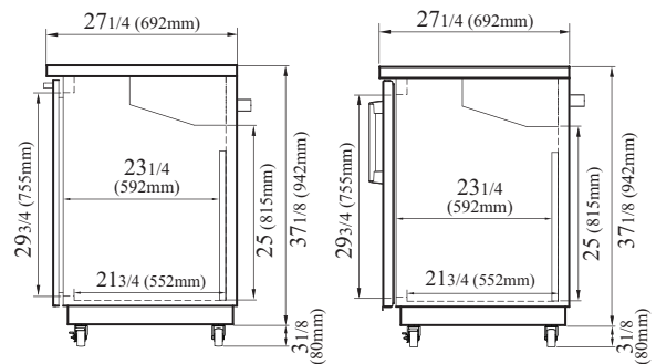
TBB-3SBD-N6 & TBB-3SGD-N SIDE VIEW
