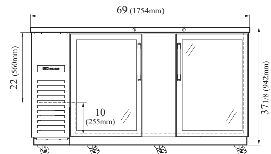
TBB-3SGD-N FRONT VIEW
