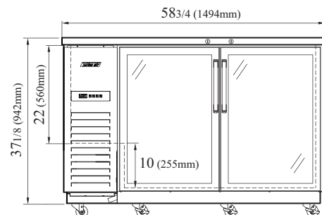
TBB-2SGD-N FRONT VIEW
