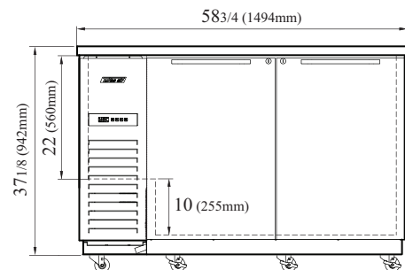
TBB-2SBD-N6 FRONT VIEW
