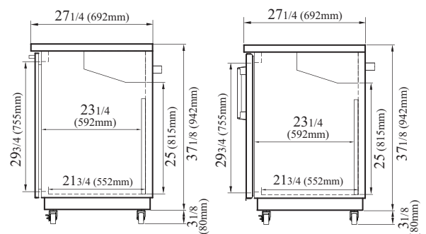
TBB-2SBD-N6 & TBB-2SGD-N SIDE VIEW
