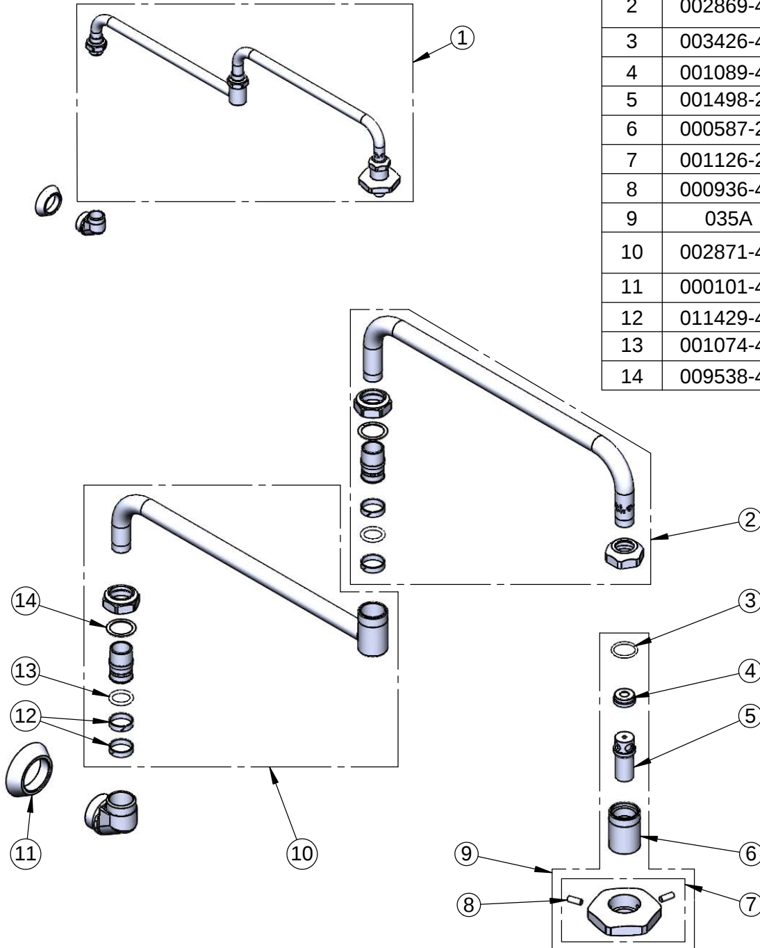
Additional View for Bill of Material Clarification
