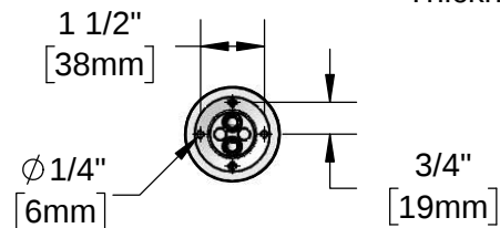
Bottom View VR Pin Hole Pattern
