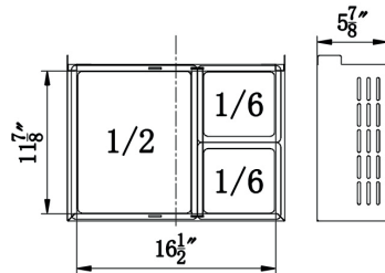
Lower drawer
