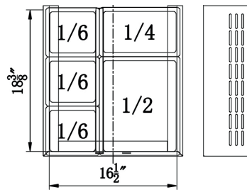
Upper drawer
