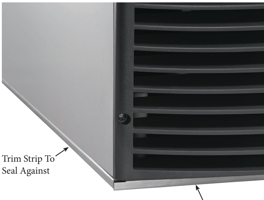
Kit Detail
