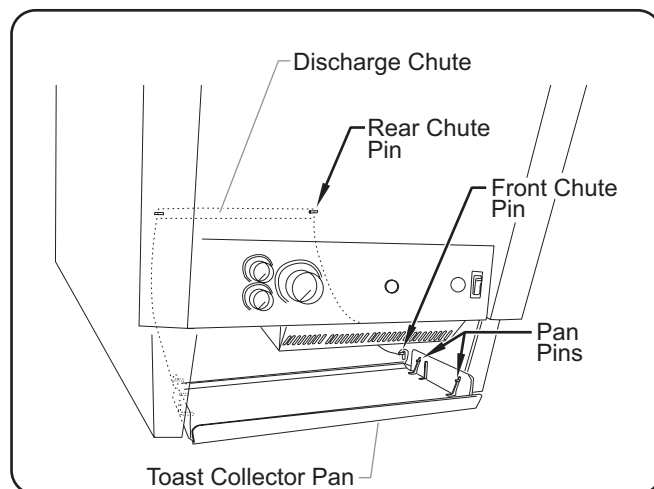
TQ-400, -800, -1200, and -1800 Series Front Discharge
