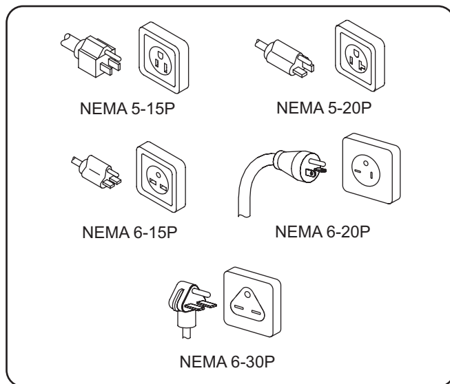
Plug Configurations
