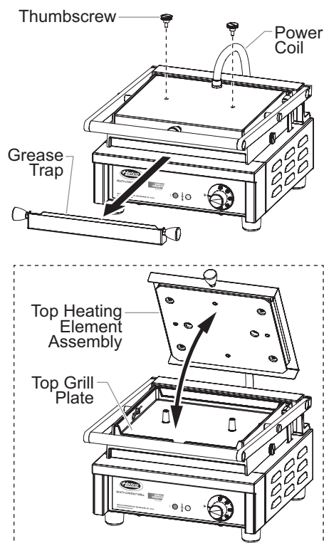
Removing Thumbscrews and the Heating Element Assembly
