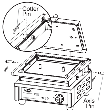
Removing the Cotter and Axis Pins
