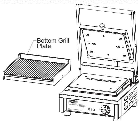
Removing the Top and Bottom Grill Plates
