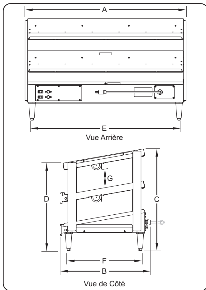
GRPWS-xxxxD Dimensions
