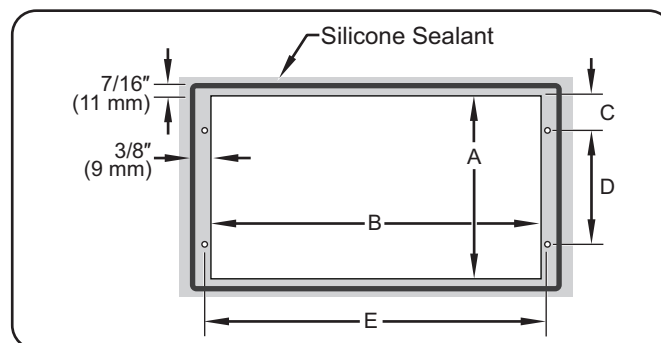
Cutout Dimensions — RMB2s
