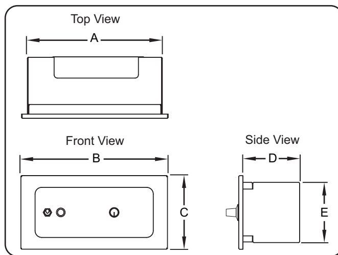
Dimensions — RMB2s
