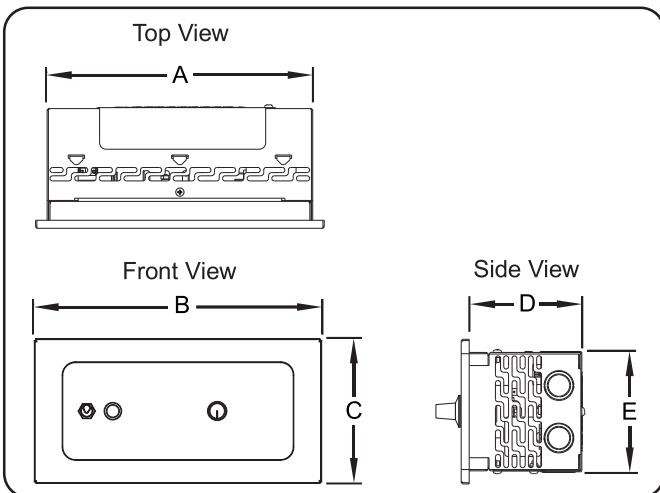
Dimensions — RMB2s
