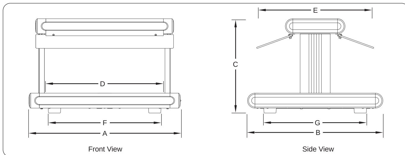
Figure 6. GR2BW Dimensions
