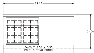
STD4464NP-12M Pan Cutout Configuration
