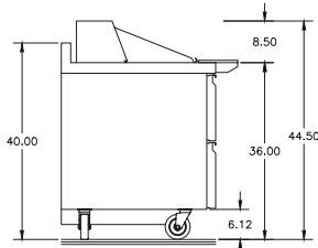
STD4464NP-18M Right Side View
