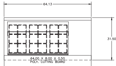
STD4464NP-18M Pan Cutout Configuration
