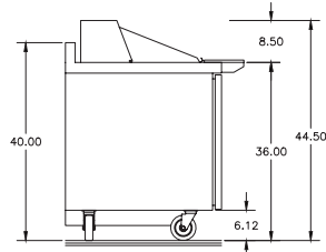
ST4464NP-18M Right Side View
