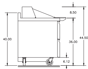
STD4464NP-12M Right Side View
