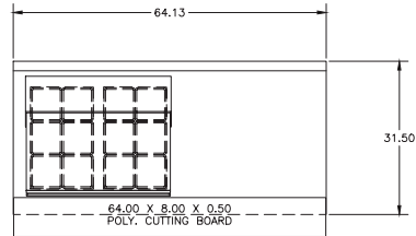
ST4464NP-12M Pan Cutout Configuration
