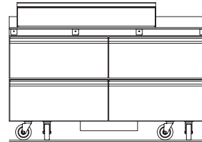
STD4464NP-18M Elevation View
