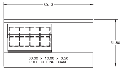
ST4460NP-8 Pan Cutout Configuration
