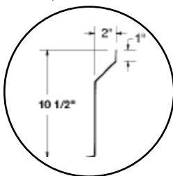
Splash Detail
