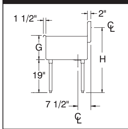
PLUMBING ROUGH-IN
